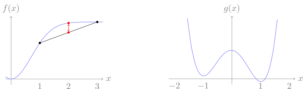
FIGURE 2: Non-convex functions. (a) f(x) = 1 - e^{-x^2} : The average of f(1) and f(3) is smaller than the value f(2) at the midpoint. Gradient descent can get stuck on the flat part. (b) g(x) = (x^2 - 1)^2 - 0.1x : Gradient descent could converge to the local minimum x_- \approx -1 or to the global one x_+ \approx 1 depending on the choice of initialization.
